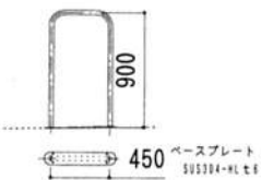
①浴室用手摺
